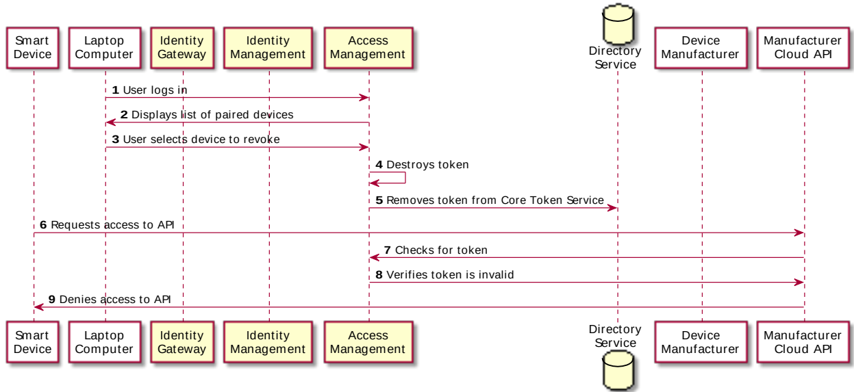
Figure 2.6. Smart Device Revocation
