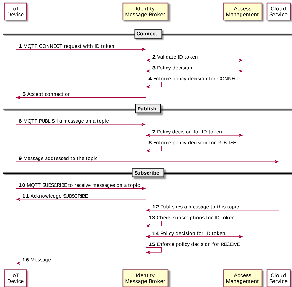
Figure 4.1. Message Broker Secures Data At the Edge
