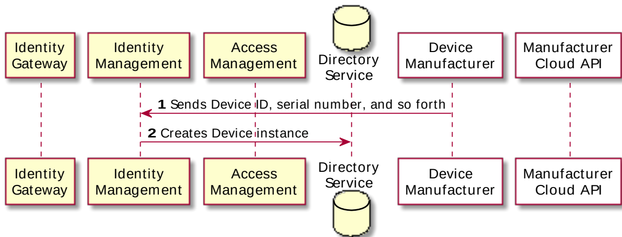
Figure 2.1. Creating and Storing a Device Identity
