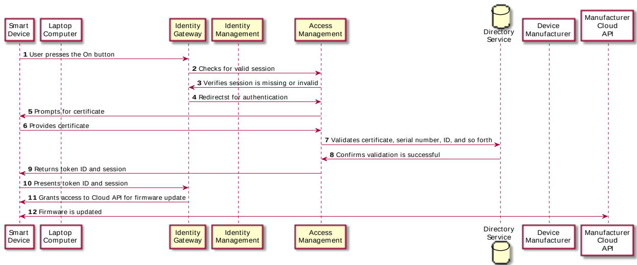
Figure 2.3. Smart Device Calls Home
