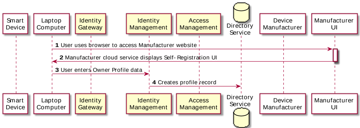
Figure 2.2. Creating a User Identity Through Self-Registration
