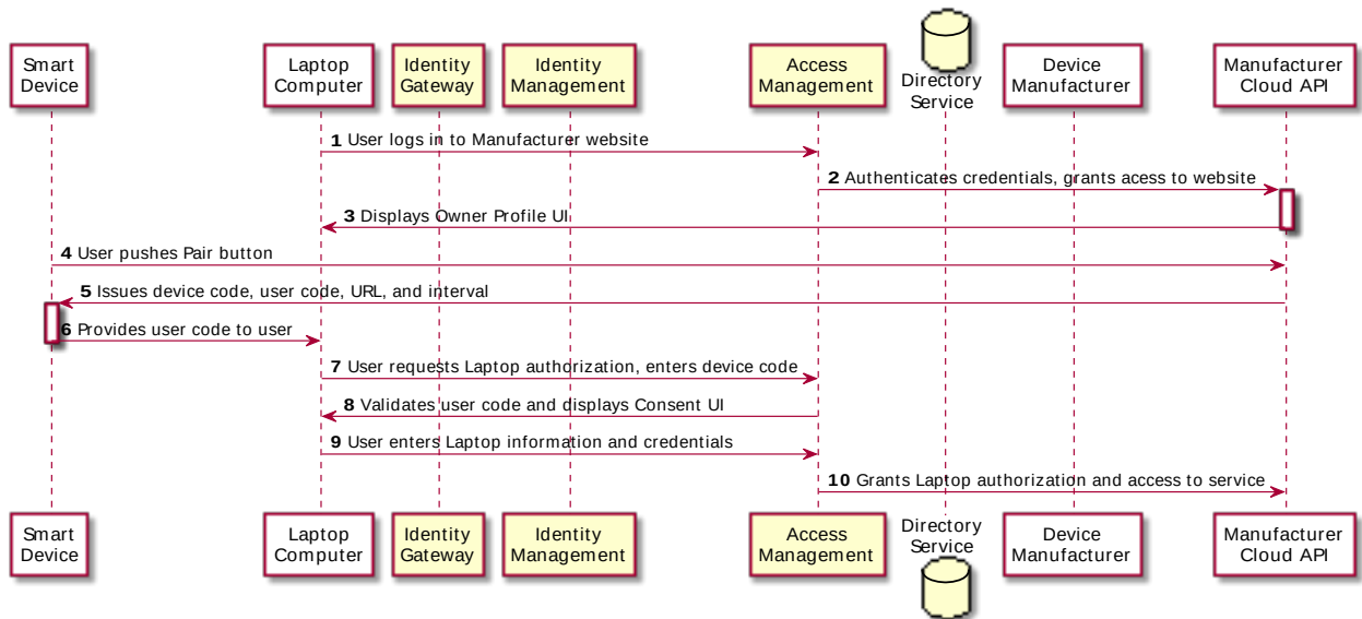
Figure 2.4. Linking User and Device Identities Using OAuth 2.0
