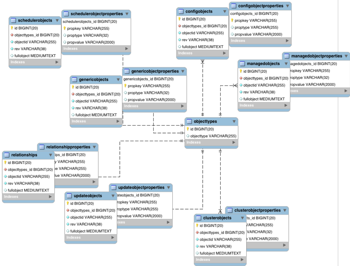
Generic Tables Entity Relationship Diagram
