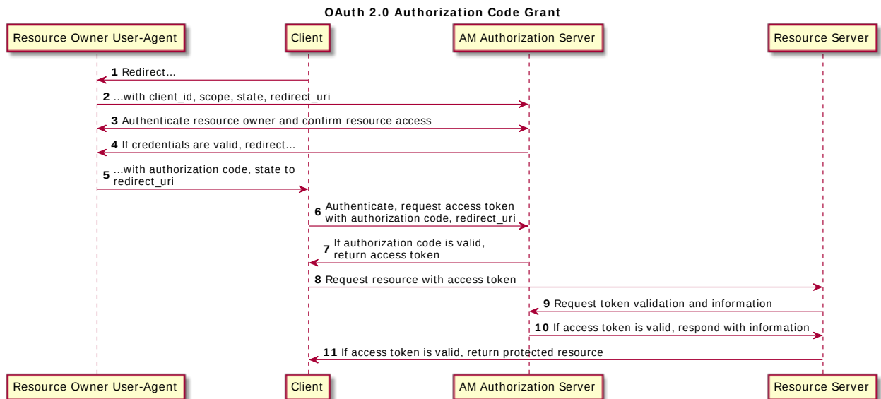
OAuth 2.0 Authorization Code Grant Process
